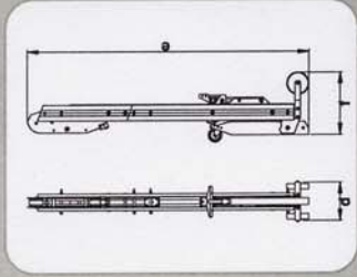
folded configuration: d = 1'- 1 1/4" e = 8'- 4 3/4" f = 1'- 10 1/4"
