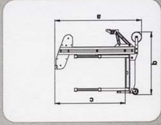
high configuration: a = 8'- 3 3/4" b = 4'- 1/4" c = 7'- 2"
