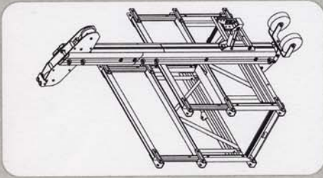
high configuration: a = 8'- 3 3/4" b = 4'- 1/4" c = 7'- 2"
