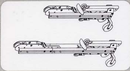
folded configuration: d = 1'- 1 1/4" e = 8'- 4 3/4" f = 1'- 10 1/4"
