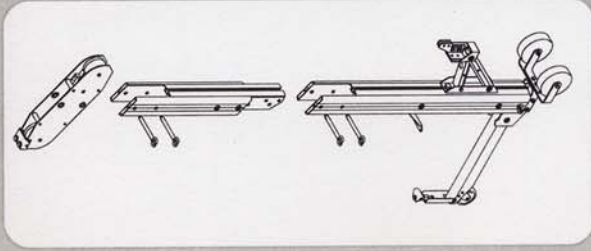
high configuration: a = 8'- 3 3/4" b = 4'- 1/4" c = 7'- 2"
